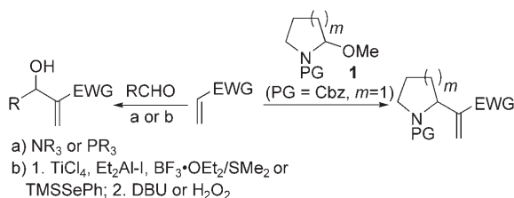
Scheme 1. The Morita–Baylis–Hillman reaction and our proposed study. Cbz = benzyloxycarbonyl, DBU = 1,8-diazabicyclo[5.4.0]undec-7-ene, TMS = trimethylsilyl, PG = protecting group.
