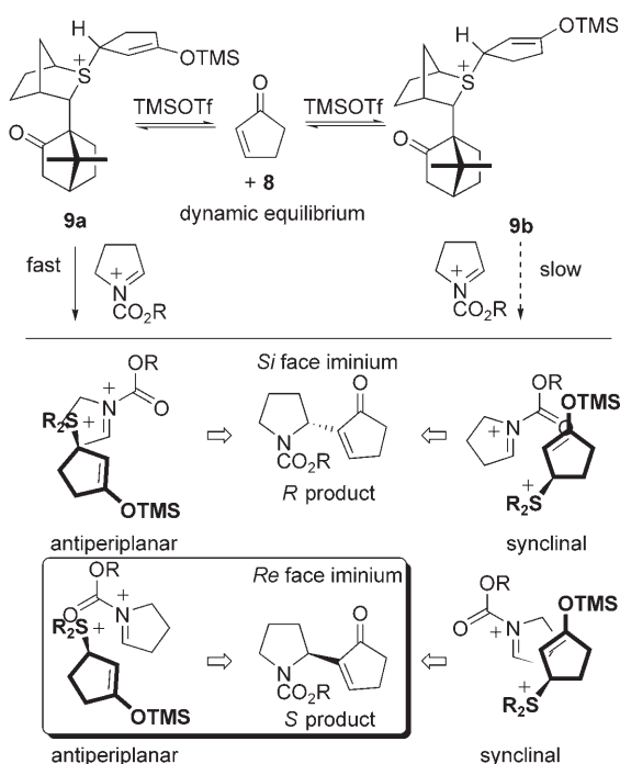
Scheme 3. Model proposed to explain the origin of the enantioselectivity.
