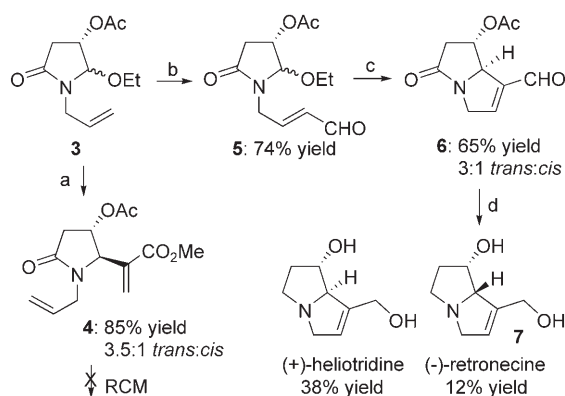
Scheme 2. Synthesis of (+)-heliotridine. a) 3 (1 equiv), methyl acrylate (3.0 equiv), TMSOTf (3.0 equiv), BF 3 ·OEt 2 (3.0 equiv), SMe 2 (3.0 equiv), CH 3 CN, RT, 24 h; b) acrolein (3.0 equiv), Grubbs–Hoveyda cat. (2 × 5 mol%), CH 2 Cl 2 , RT, 12 h; c) TMSOTf (3.0 equiv), BF 3 ·OEt 2 (3.0 equiv), SMe 2 (3.0 equiv), CH 3 CN, RT, 3 h; d) LiAlH 4 (7.0 equiv), THF, reflux, 1 h.
